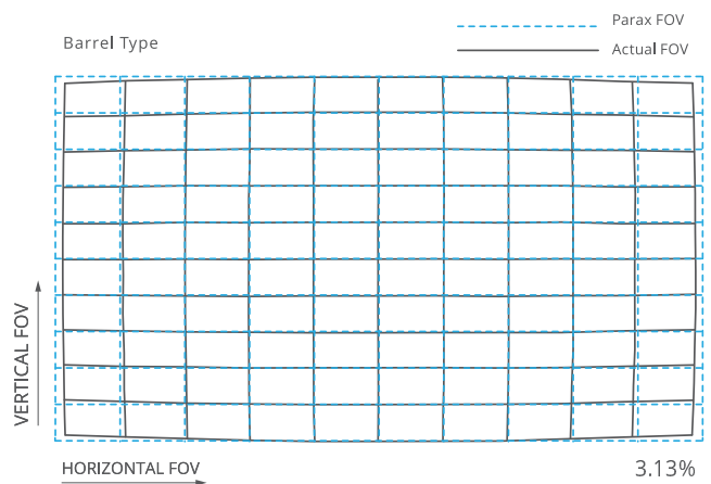
Irix 11mm f/4.0 DISTORTION
